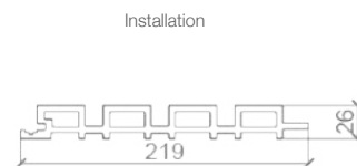
Section View
