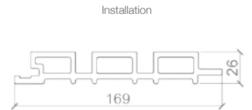
Section View
